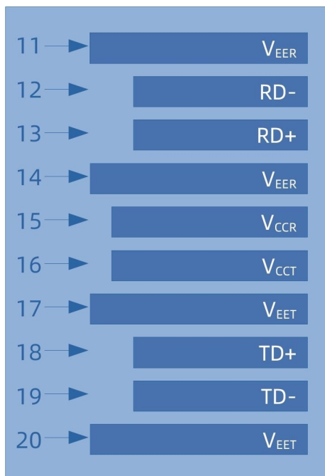
Top View of Board
